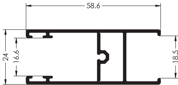
Ref. 6033 HOJA CRISTAL CLIMALIT
