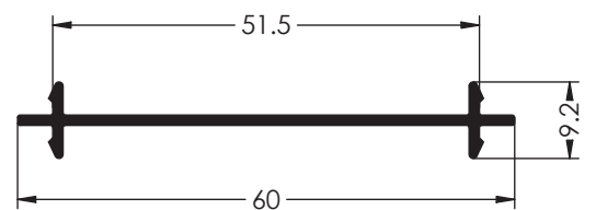
Ref. 6068 UNION CERCOS
