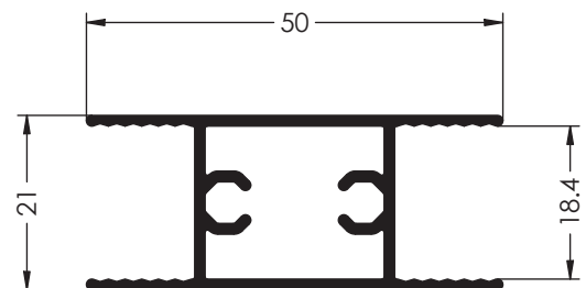
Ref. 6062 PARTELUNAS CLIMALIT
