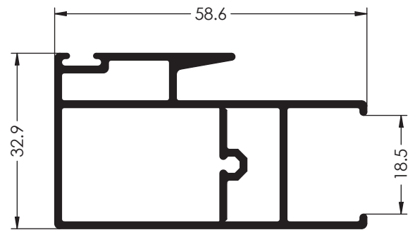
Ref. 6031 HOJA CENTROS CLIMALIT
