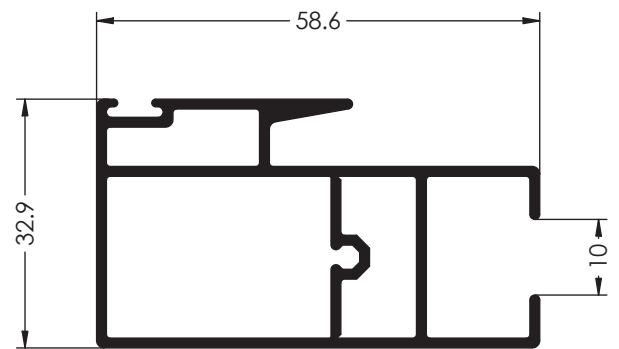
Ref. 6032 HOJA CENTROS CRISTAL MONOLITICO
