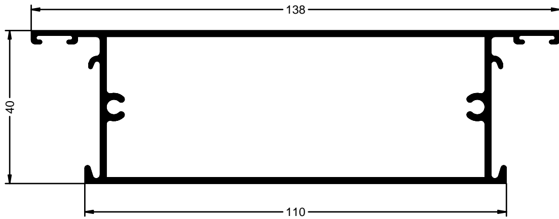
ZOCALO CENTRAL
