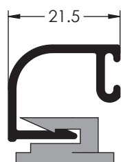
Ref. 1688 JUNQUILLO
