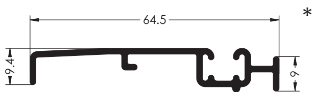
Ref. 6006 UNION DE CERCOS
