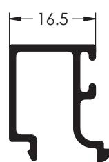
Ref. 1617 JUNQUILLO
