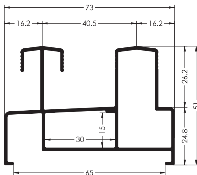
Ref. 6009 CERCO 73 mm
