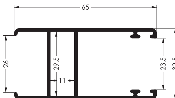
Ref. 6127 HOJA
