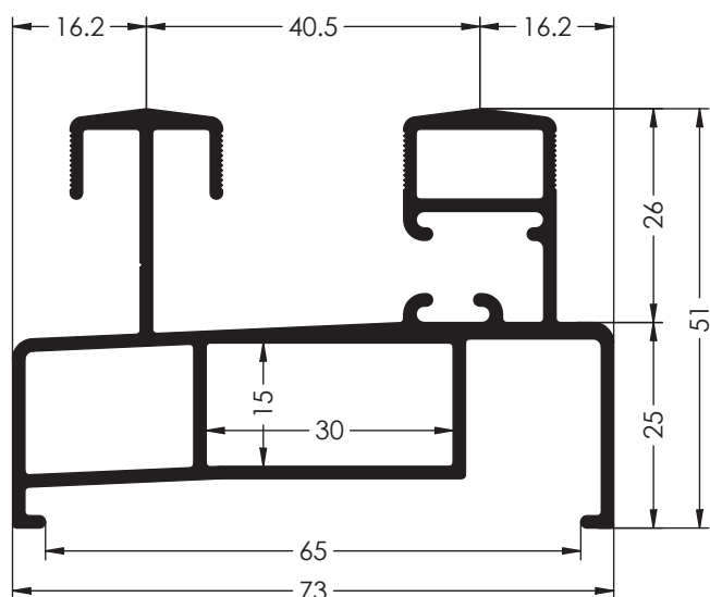
Ref. 6000 CERCO 73 mm
