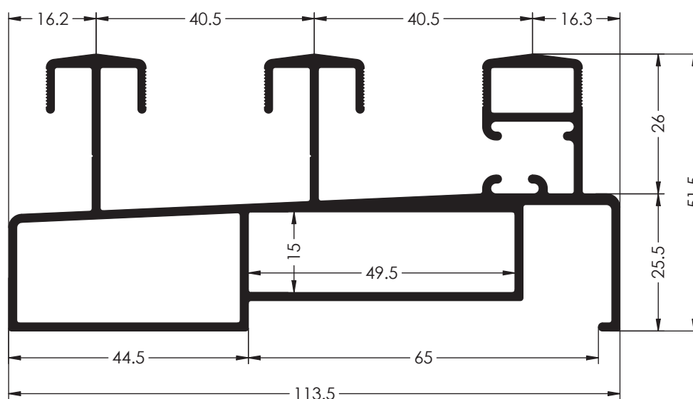
Ref. 6020 CERCO 3 CARRILES
