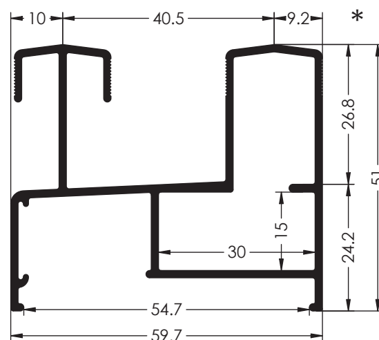
Ref. 6014 CERCO 60
