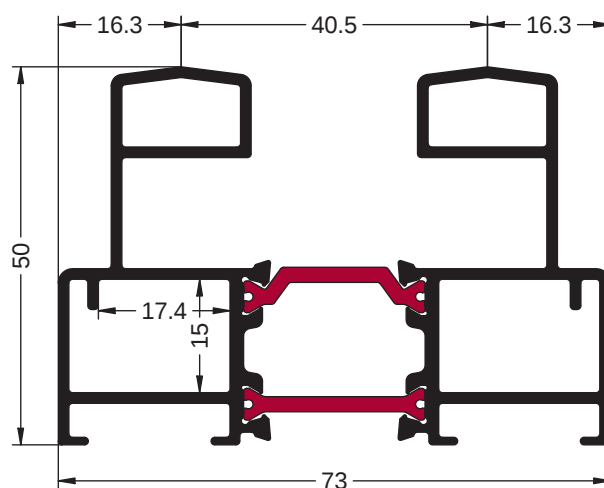
Ref. 9744 MARCO PERIMETRAL
