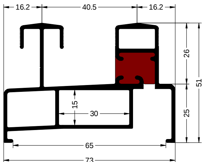
Ref. 9000 CERCO 73 mm
