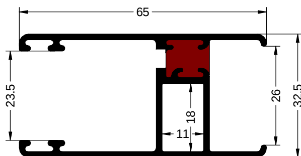
Ref. 9001 HOJA 65 mm
