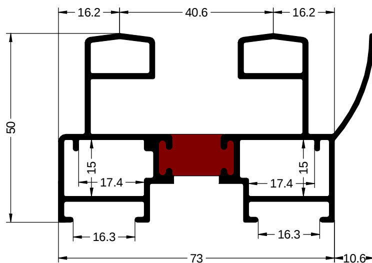
Ref. 9016 CERCO S/EURO PLUS
