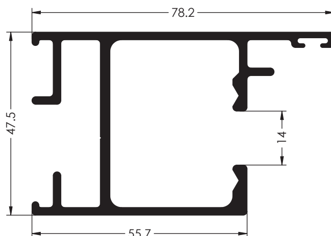
Ref. 1679 CERCO SUPERIOR
