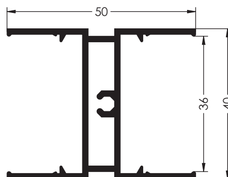
Ref. 2445 DIVISION HOJAS MALLORQUINA
